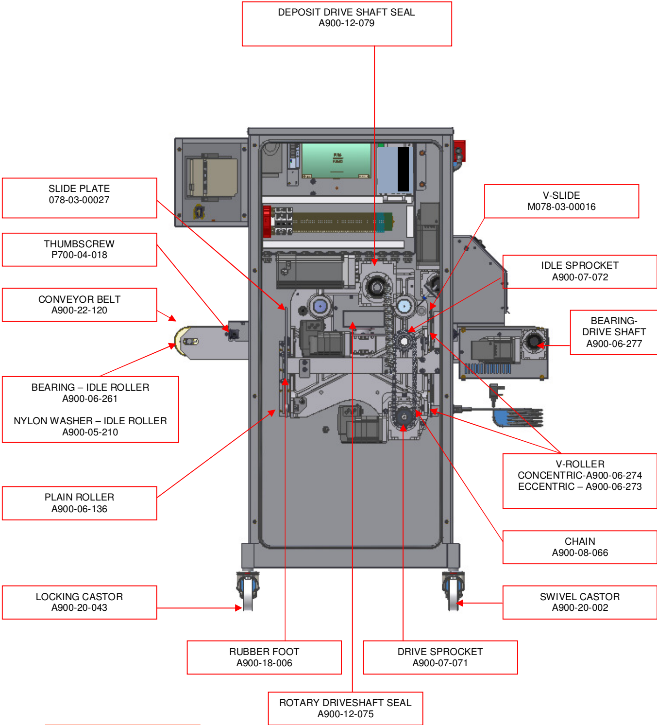
REAR VIEW WITH COVER REMOVED
